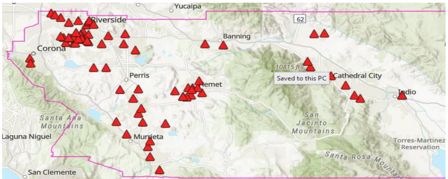
ILI-related EMS response in Riverside County, ePCR distribution map: Week 36
