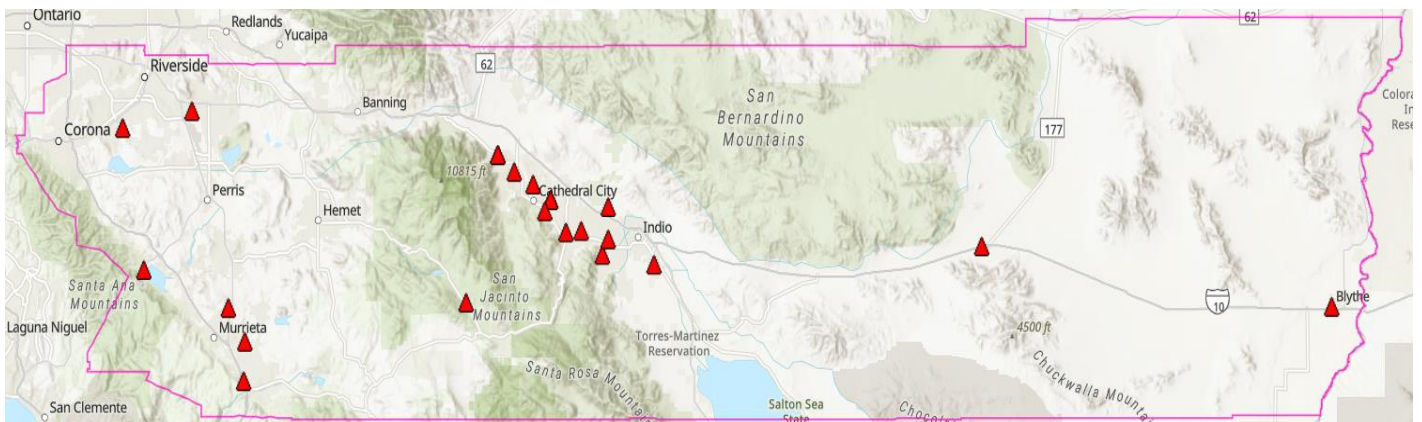
Heat-related EMS response in Riverside County, ePCR distribution map: Week 36
