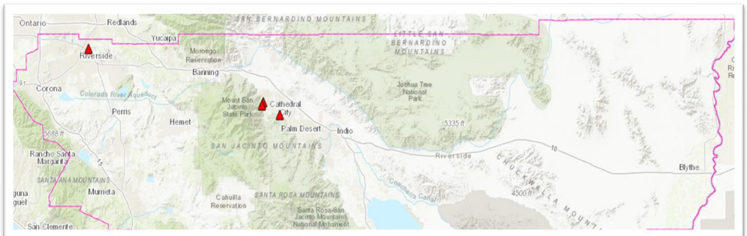
Heat-related EMS responses in Riverside County, ePCR distribution map: Week 16
