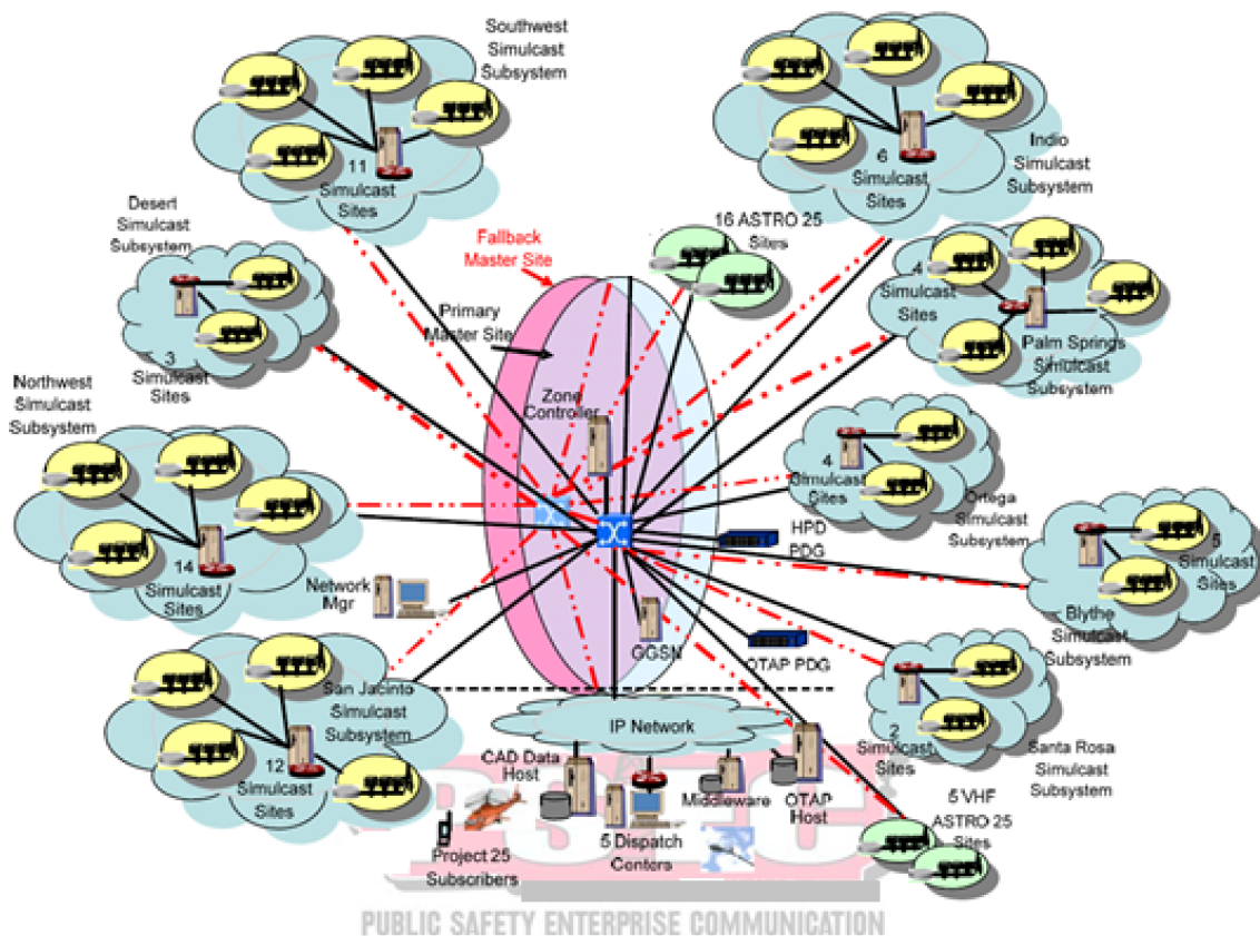
Figure 16: PSEC System Architecture
